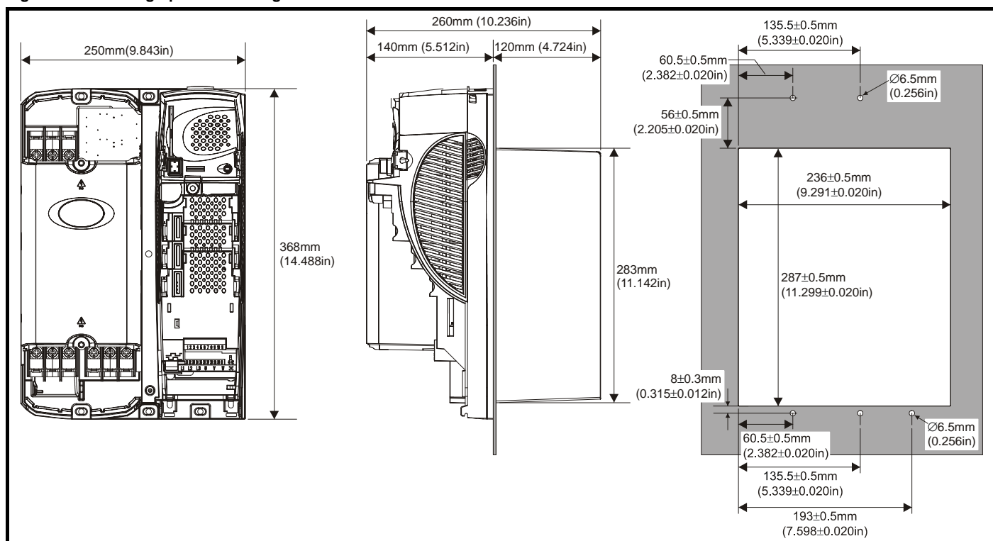
Figure 3-33 Through-panel mounting the size 4 drive
