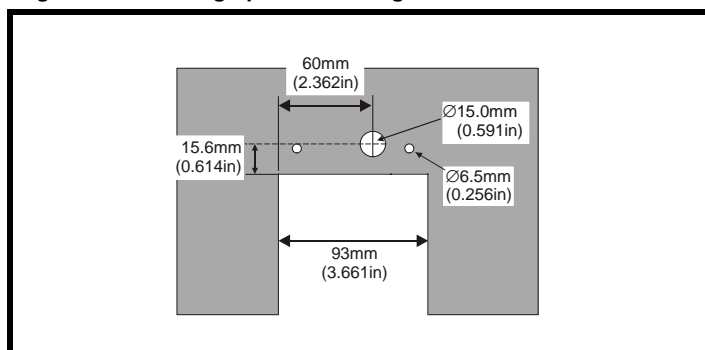
Figure 3-55 Through-panel mounting cut-out details for size 1
