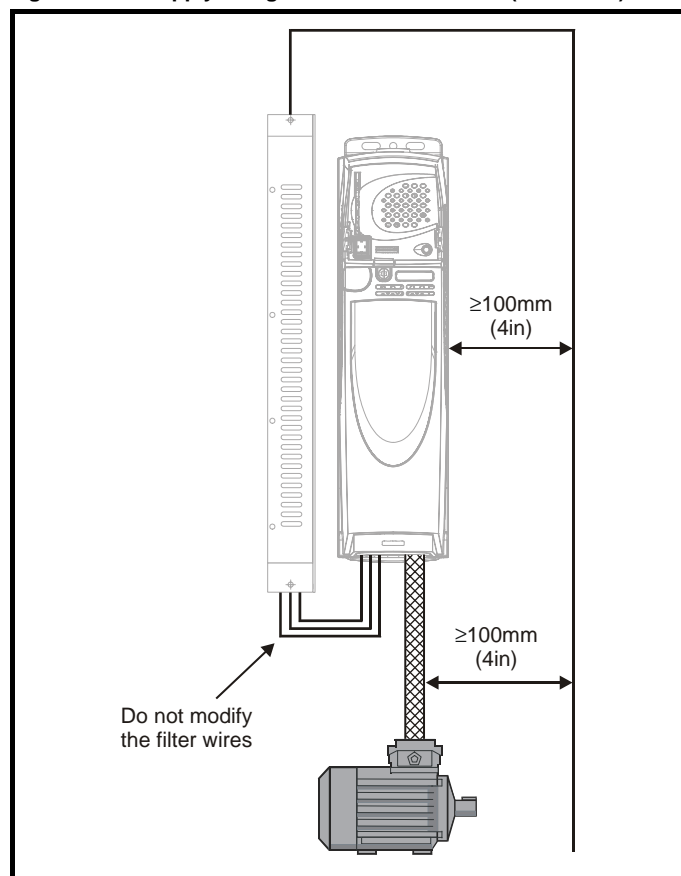
Figure 4-30 Supply and ground cable clearance (size 1 to 3)
