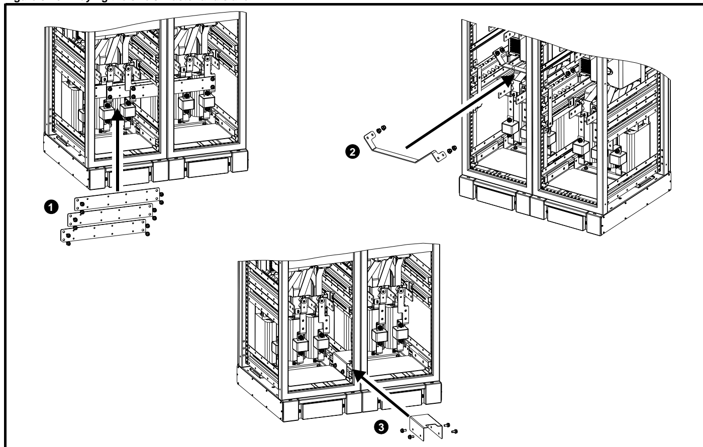
Figure 3-16 Baying the size 9 master and slave
