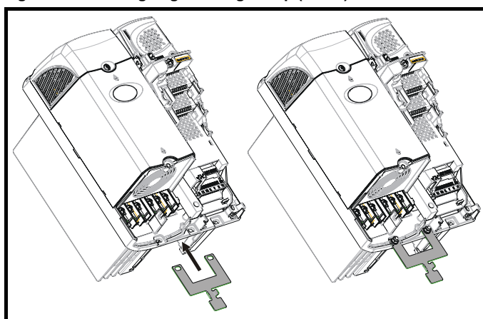
Figure 4-21 Fitting of grounding bracket (sizes 1 to 6)
