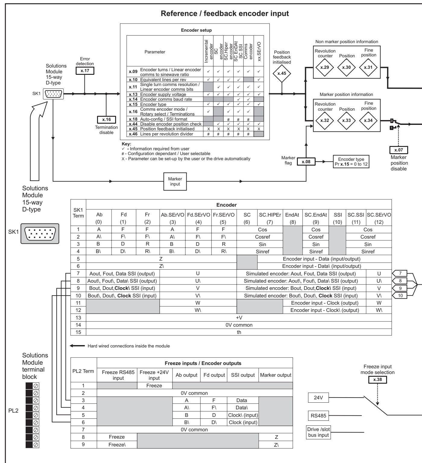
11.15.2 Feedback module category Figure 11-24 SM-Universal Encoder Plus logic diagram
