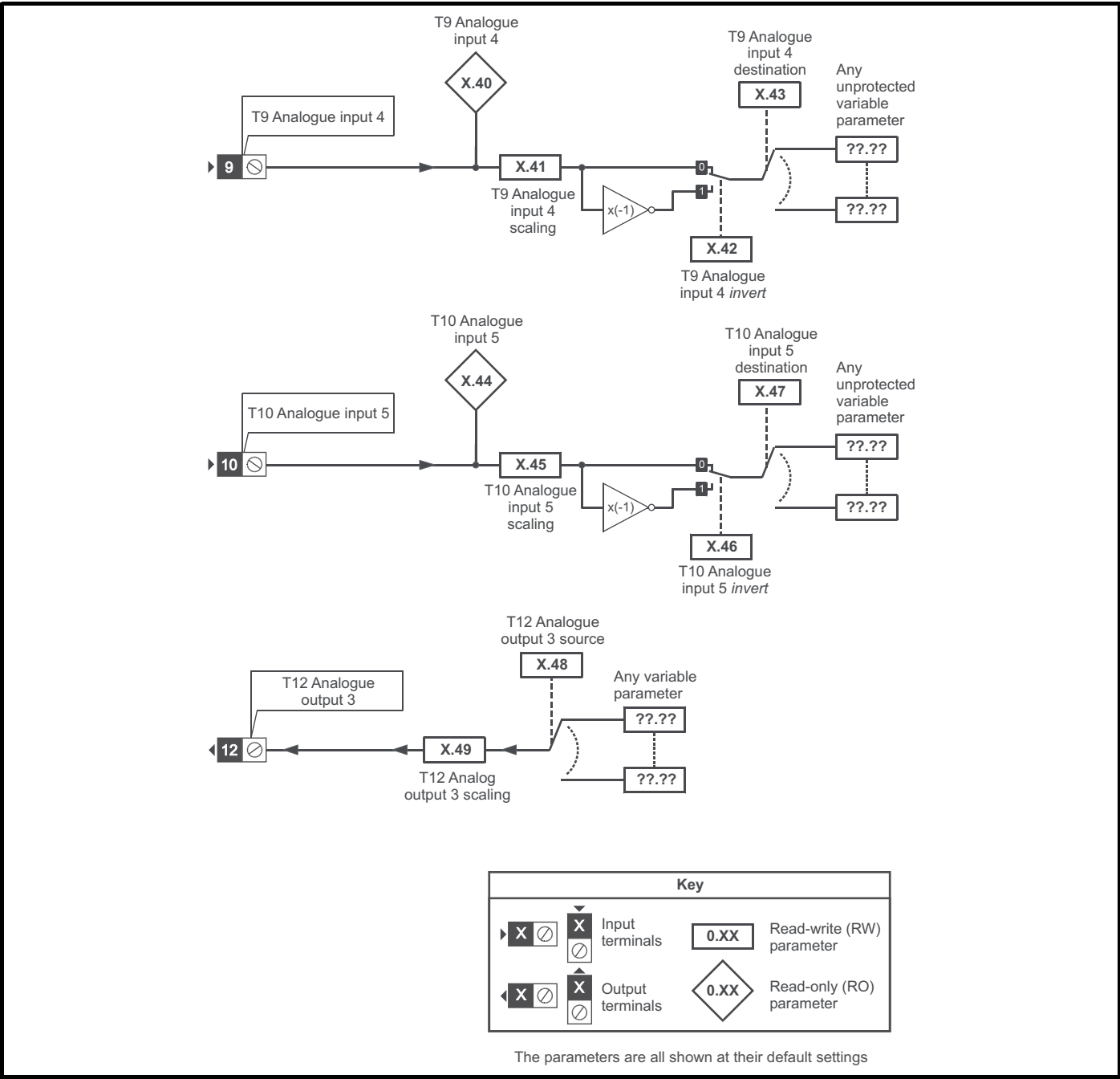
11.15.3 Automation module category Figure 11-27 SM-I/O Plus analogue logic diagram
