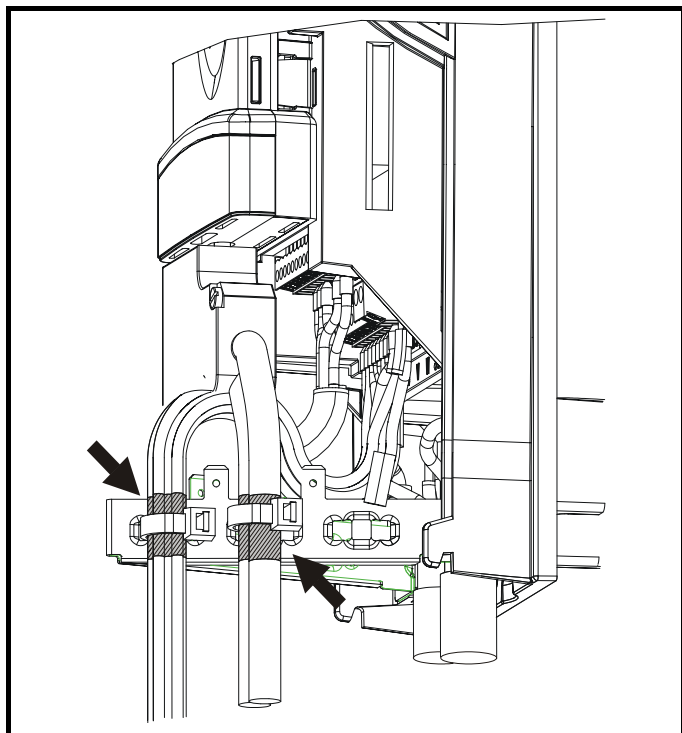
Figure 4-36 Grounding of signal cable shields using the grounding bracket
