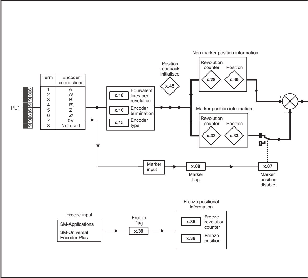
Figure 11-26 SM-Encoder Plus logic diagram
