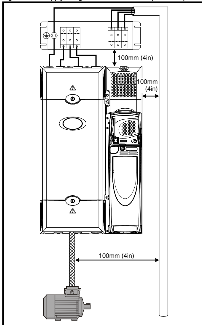
Figure 4-31 Supply and ground cable clearance (size 4 to 6)
