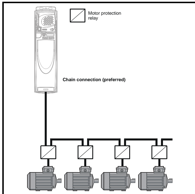
Figure 4-16 Preferred chain connection for multiple motors
