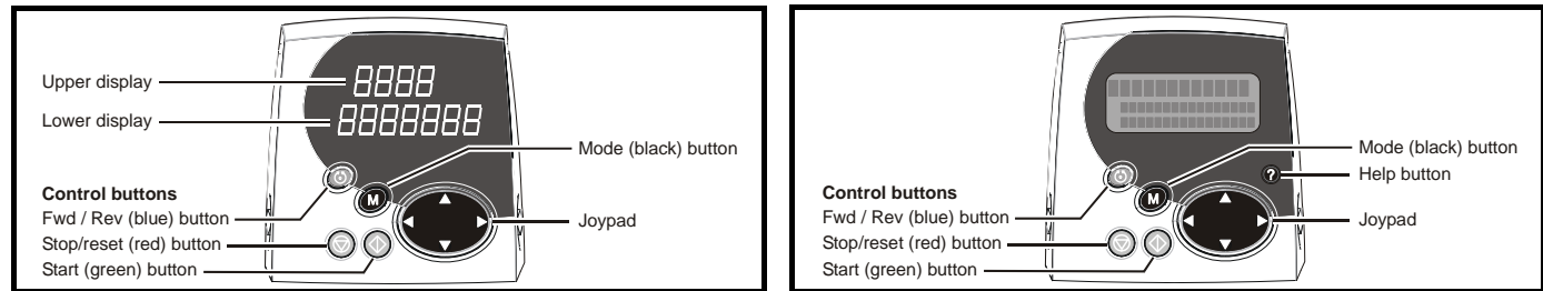
Figure 5-1 SM-Keypad
