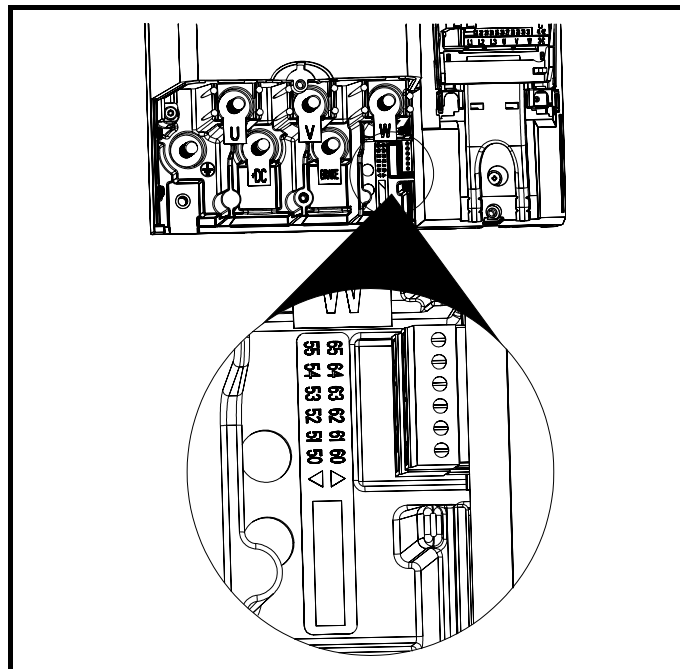
Figure 4-45 Size 4 and 5 low voltage DC mode enable connections
