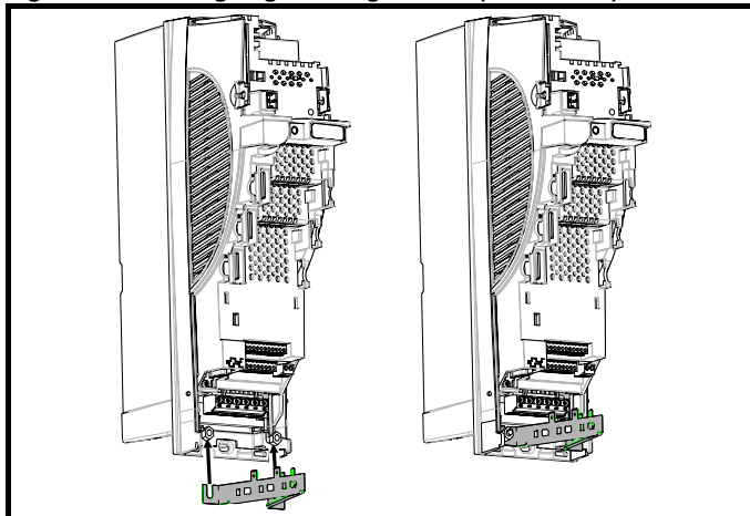
Figure 4-21 Fitting of grounding bracket (sizes 1 to 6)
