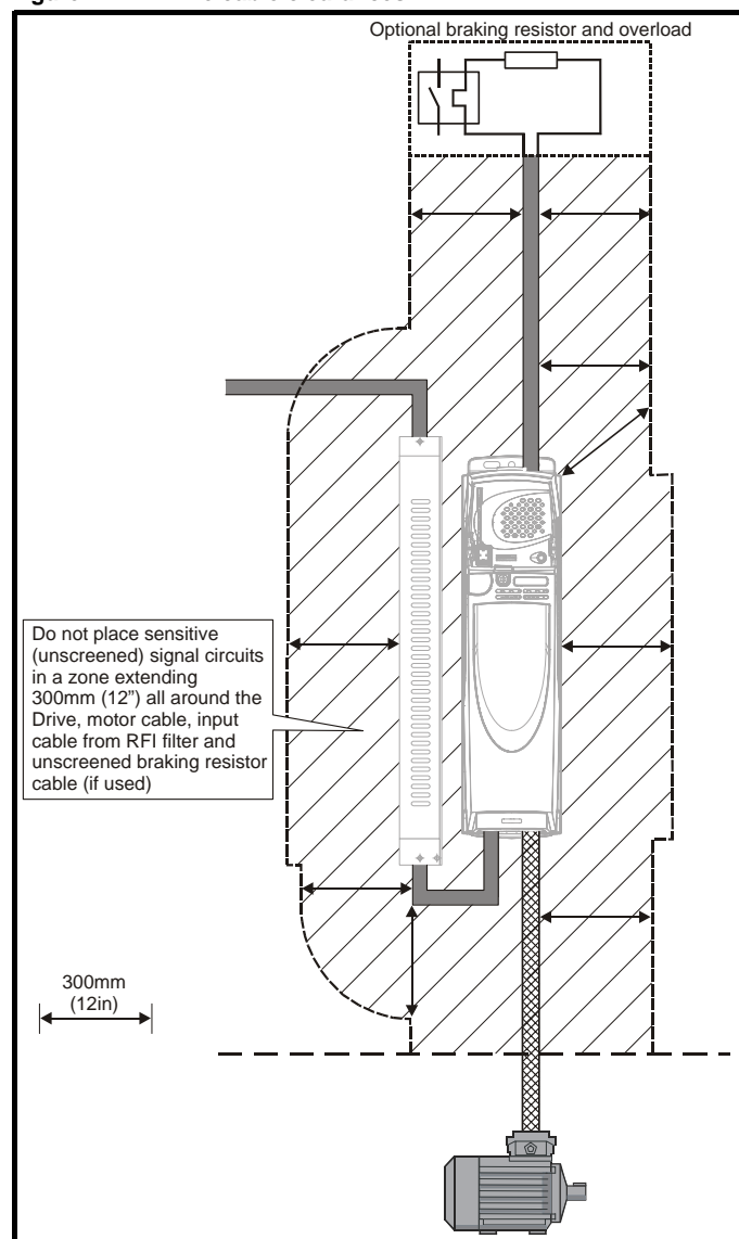
Figure 4-27 Drive cable clearances
