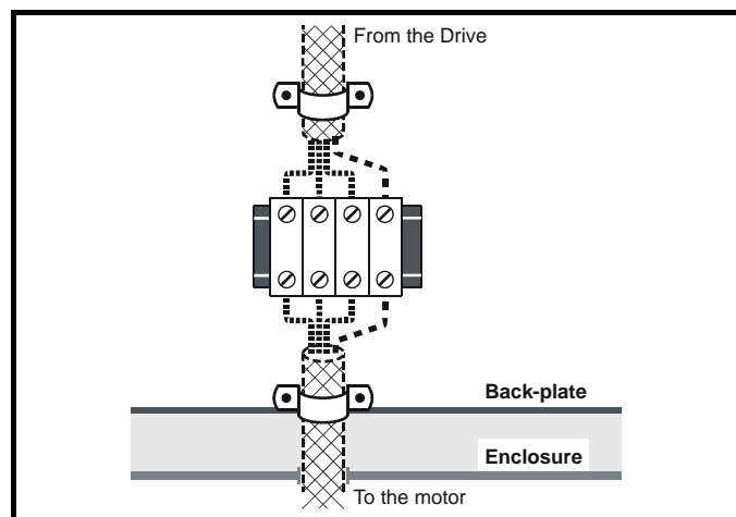
Figure 4-37 Connecting the motor cable to a terminal block in the enclosure
