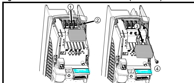
Figure 4-24 Removal of internal EMC filter (size 1 to 3)
