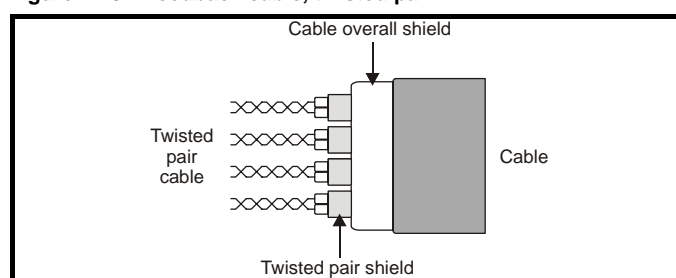
Figure 4-28 Feedback cable, twisted pair
