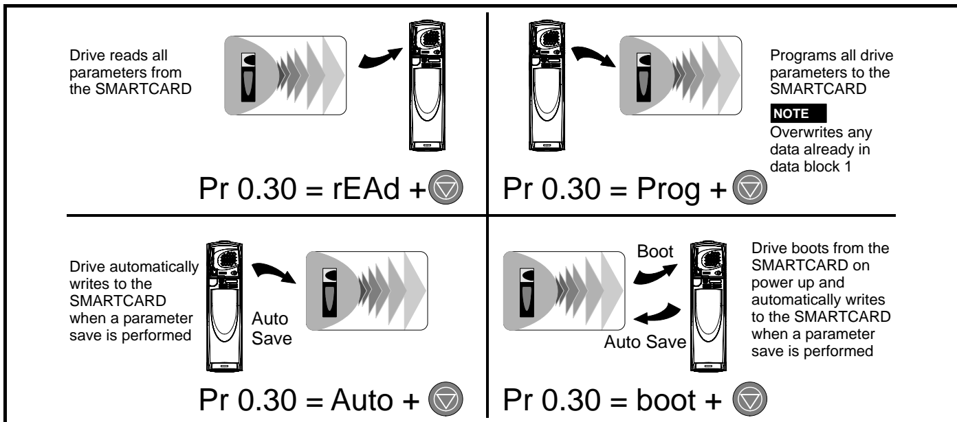
Figure 9-2 Basic SMARTCARD operation
