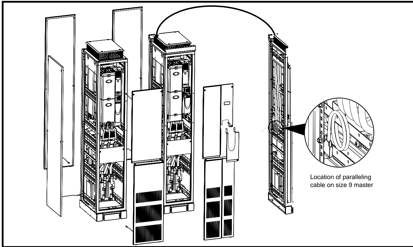
Figure 3-13 Preparation for baying the size 9 free standing drive (slave and master)
