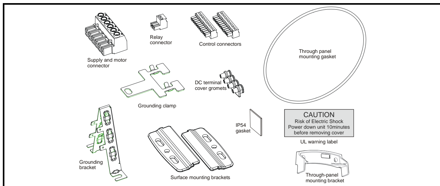
Figure 2-5 Accessories supplied with size 1
