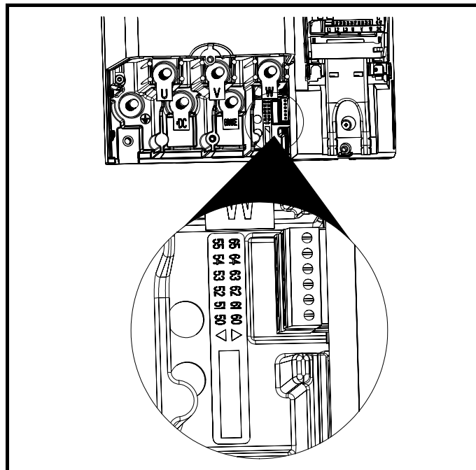
Figure 4-12 Size 6 heatsink fan supply connections
