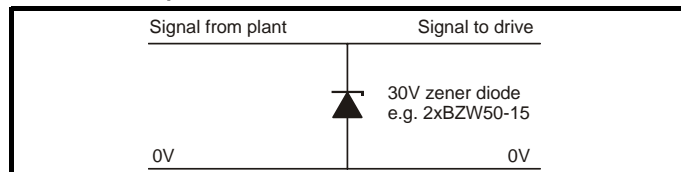
Figure 4-40 Surge suppression for analogue and bipolar inputs and outputs
