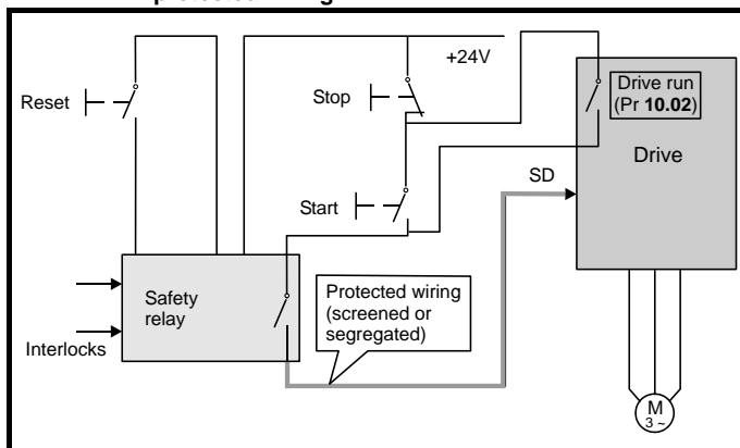
Figure 4-49 Category 3 interlock using Secure Disable with protected wiring
