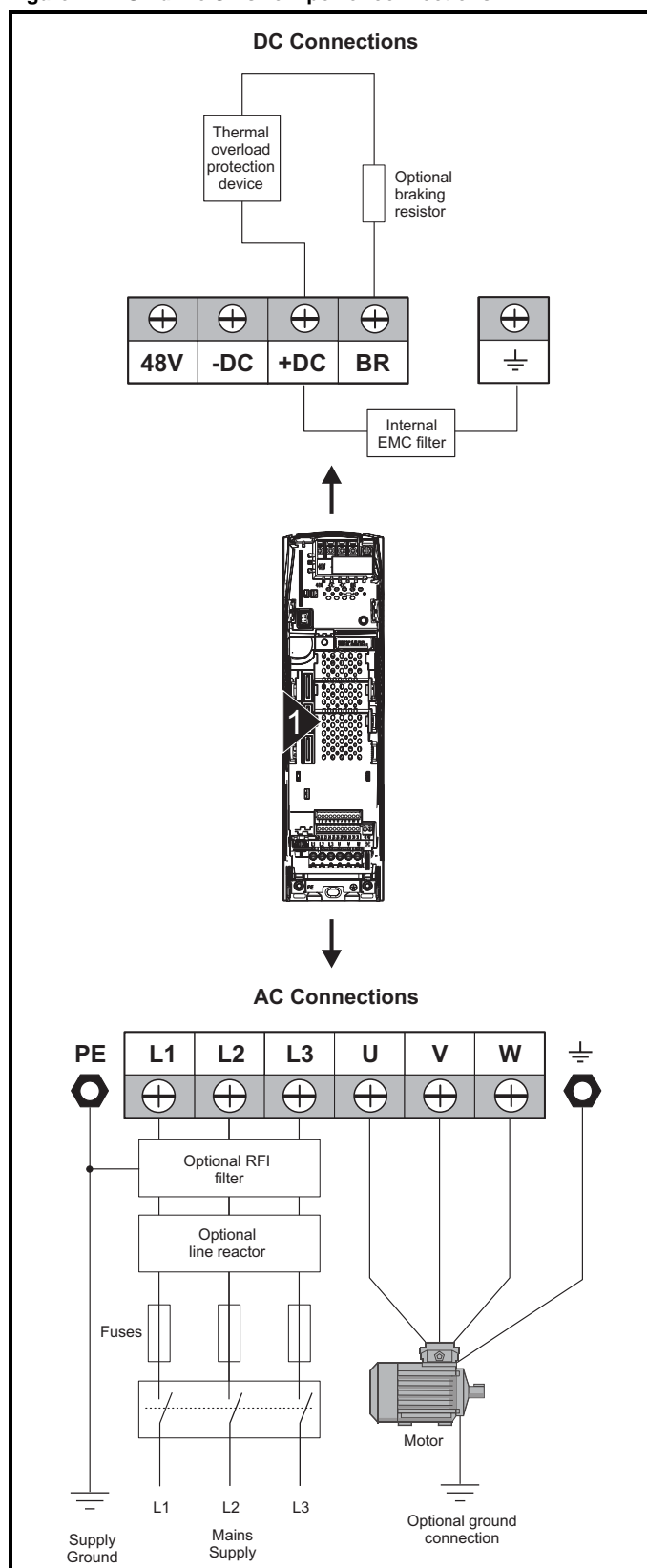
Figure 4-1 Unidrive SP size 1 power connections
