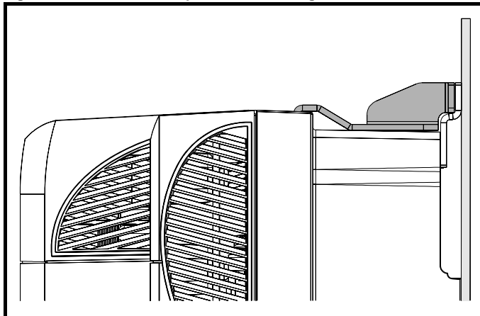
Figure 3-38 Location of top surface mounting brackets for size 5 and 6
