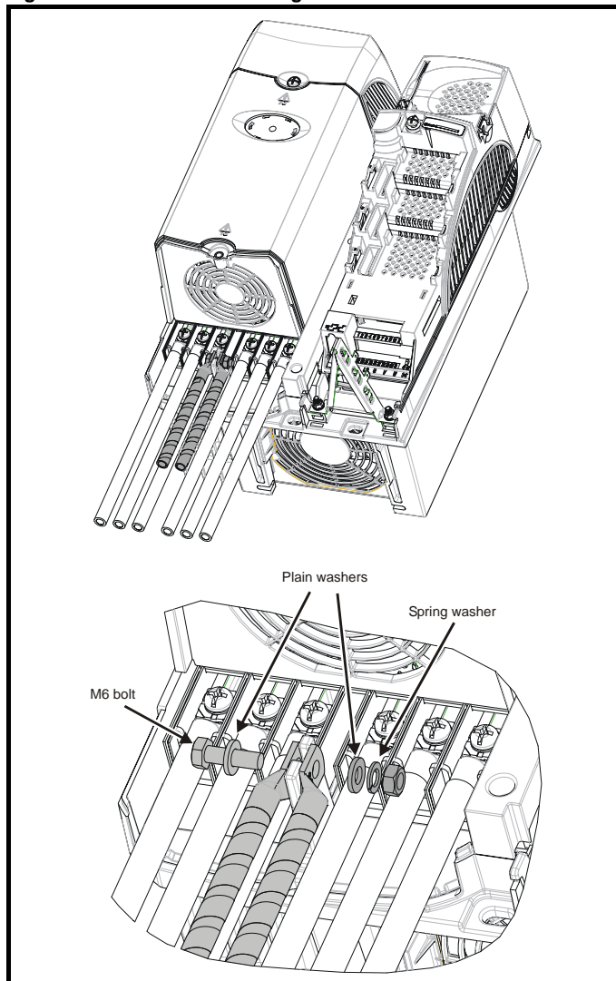
Figure 4-9 Unidrive SP size 4, 5 and 6 ground connections
