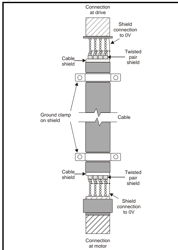
Figure 4-29 Feedback cable connections
