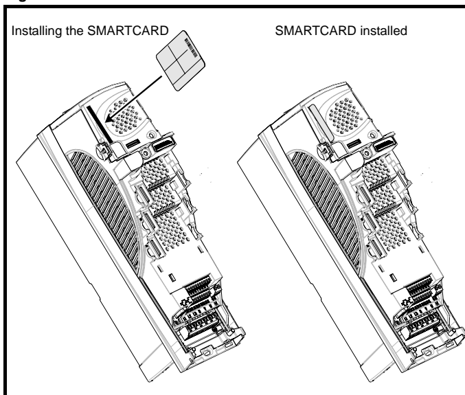
Figure 9-1 Installation of the SMARTCARD
