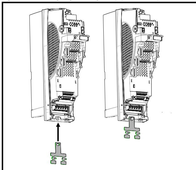
Figure 4-20 Fitting of grounding clamp (size 3)
