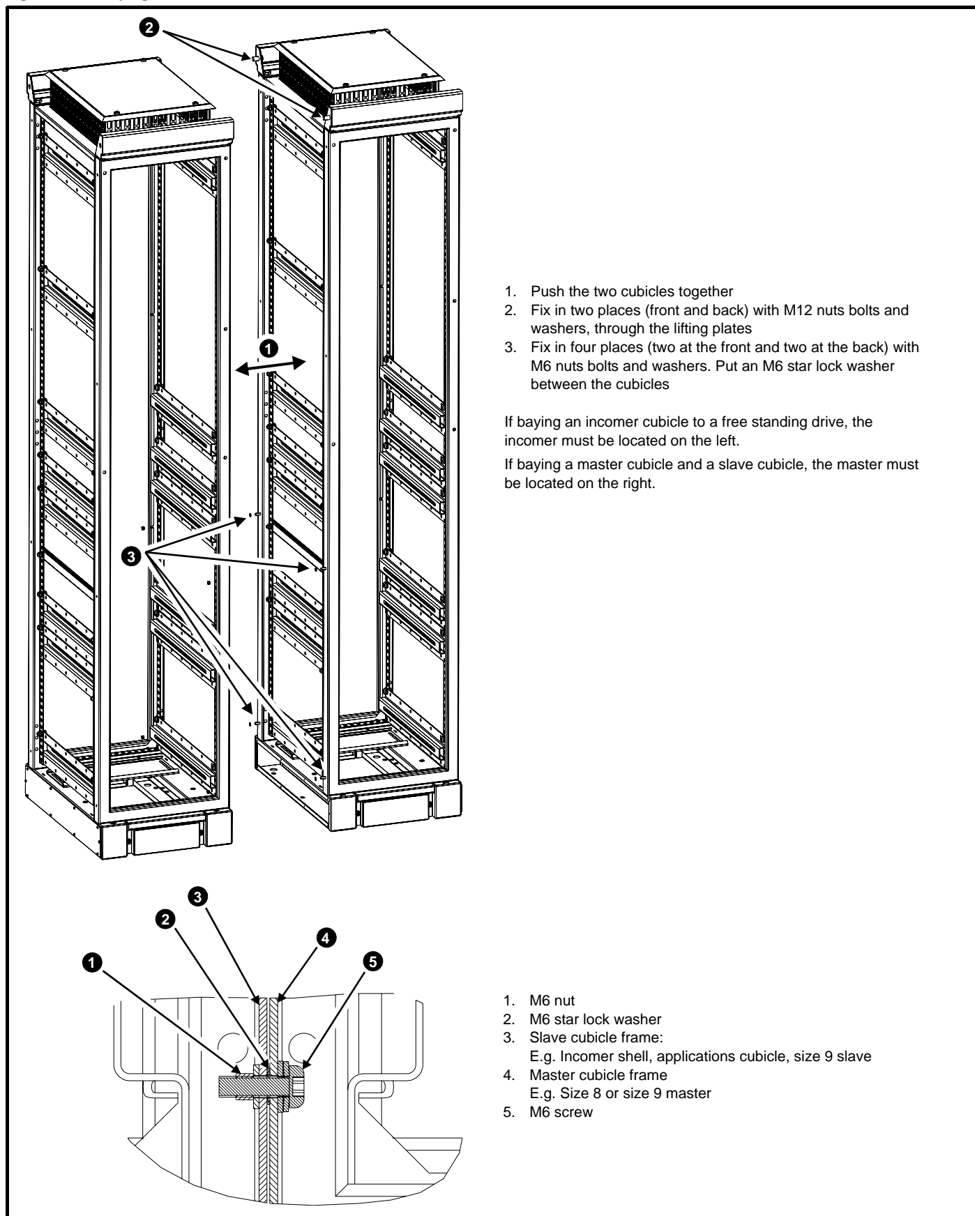
Figure 3-14 Baying of cubicles
