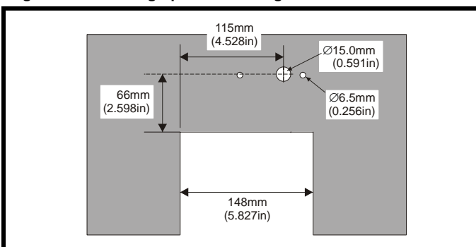
Figure 3-56 Through-panel mounting cut-out details for size 2
